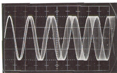
Figure 7 - Modulation FM
