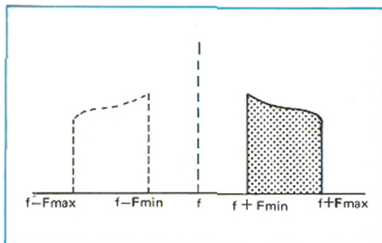
Figure 5 - Transmission BLU
