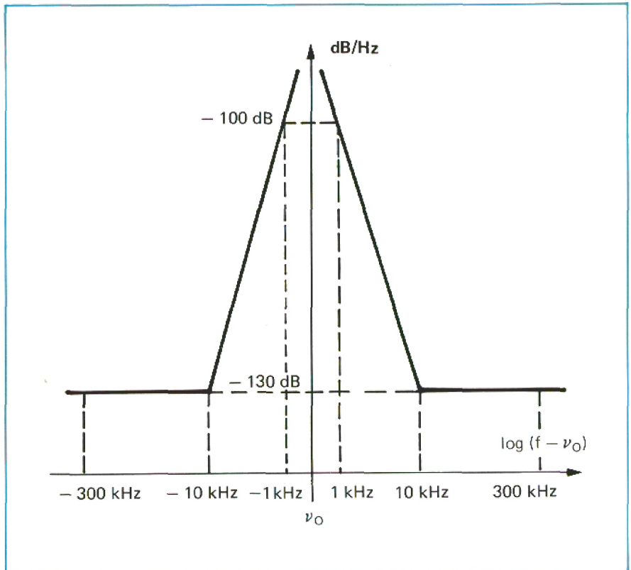
Figure 3 - Exemple de spectre RF
